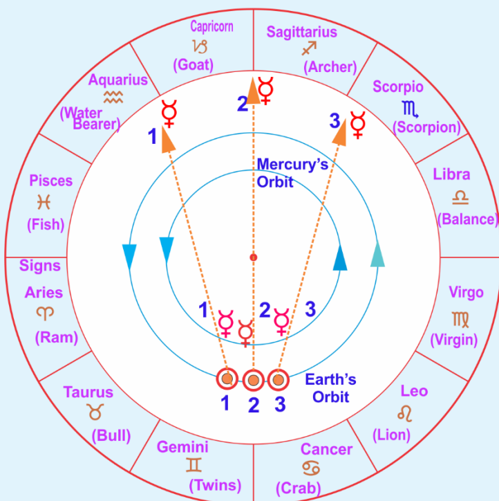
Retrograde Motion of the Inner Planet
