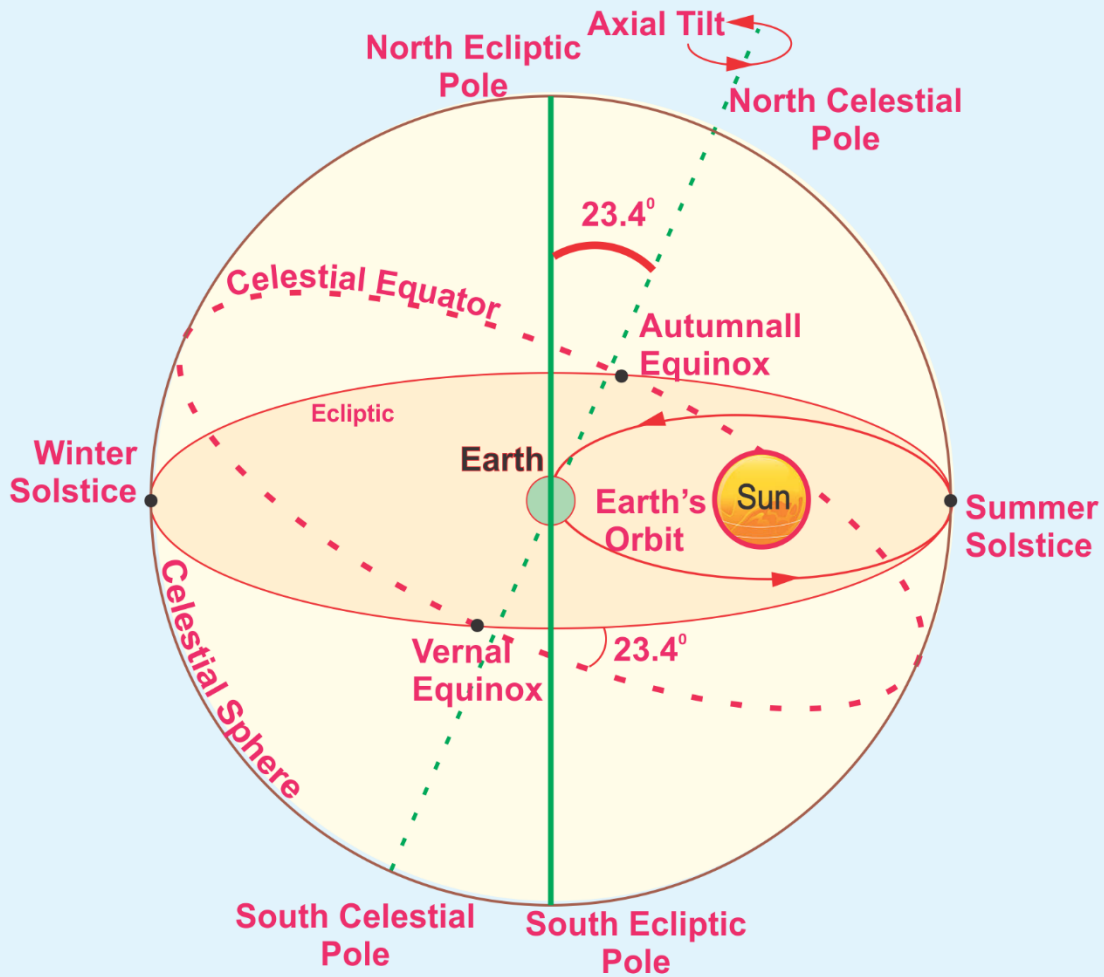
Celestial Sphere, Ecliptic and the Sun
