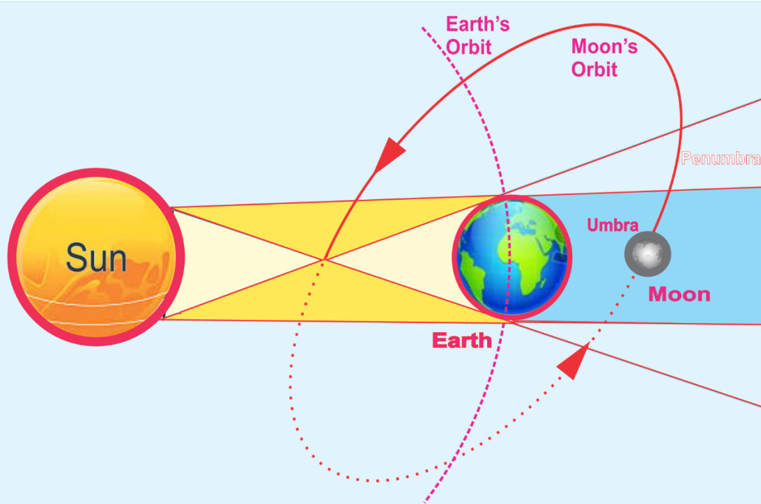
Lunar Eclipse
