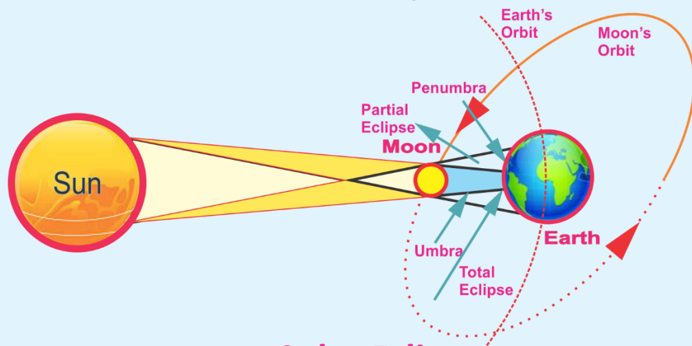
Solar Eclipse
