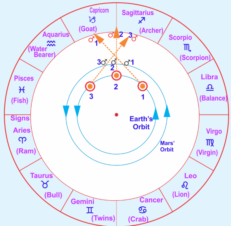
Retrograde Motion of the Outer Planet
