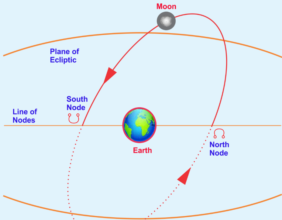
The Moon's Node
